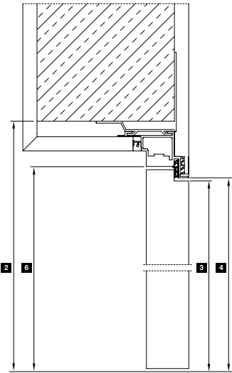
Vertical view with reverse-opening door leaf
